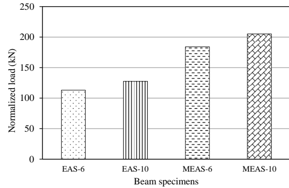
Figure 13. Comparison of normalized load (effect of reinforcement ratio)
