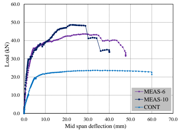
Figure 11. Load versus deflection curves of beams (Group A and C)
