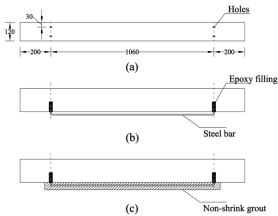
Figure 3. Epoxy anchorage system (mm)
