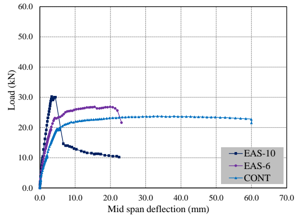
Figure 10. Load versus deflection curves of beams (Group A and B)
