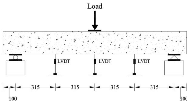
Figure 8. Schematic of loading setup (mm)
