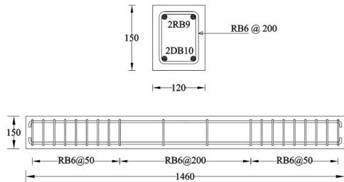
Figure 1. Beam specimen details (mm)
