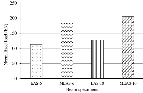
Figure 12. Comparison of normalized load (effect of anchorage system)
