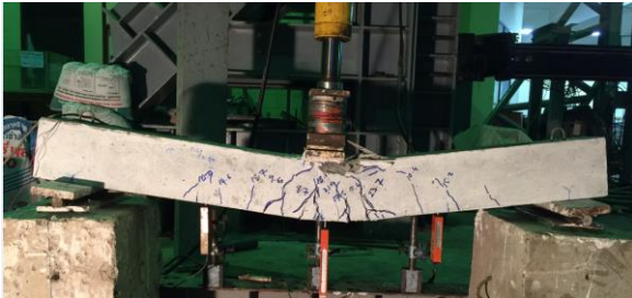
Figure 14. Failure mode of control beam
