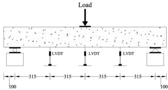
Figure 8. Schematic of loading setup (mm)
